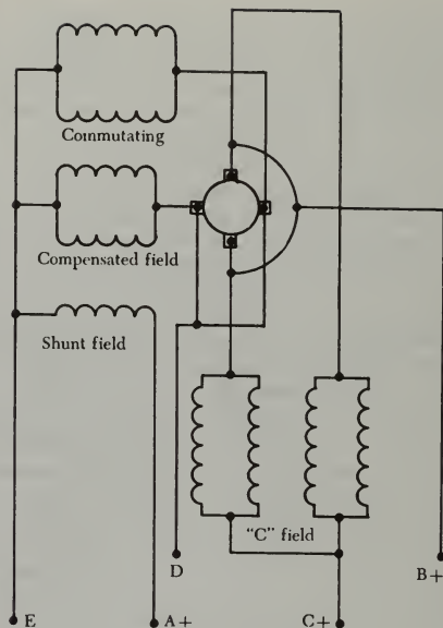
FIGURE 5-14. Starter-generator internal circuit.
